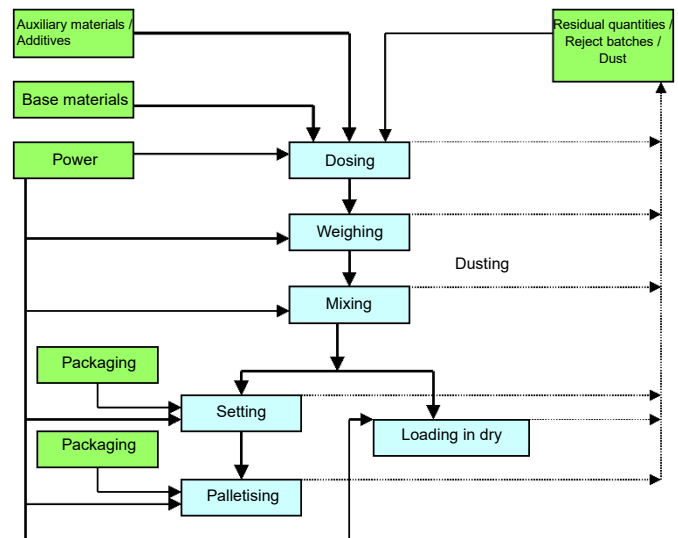
Fig. 1: Manufacturing process (green: input; blue: uniform process)
