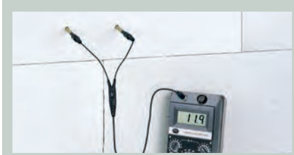
APPLICATION Measuring structural moisture using the RTU 600 unit and an M 21-100 deep measuring electrode pair
